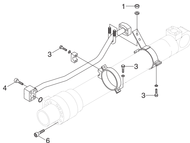
ARM CYLINDER
