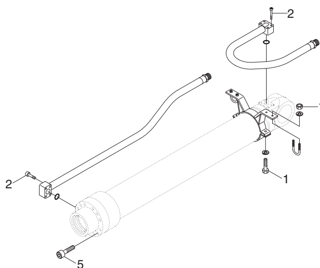
BUCKET CYLINDER (LONG REACH)
