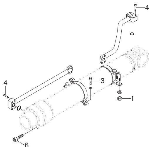
BUCKET CYLINDER
